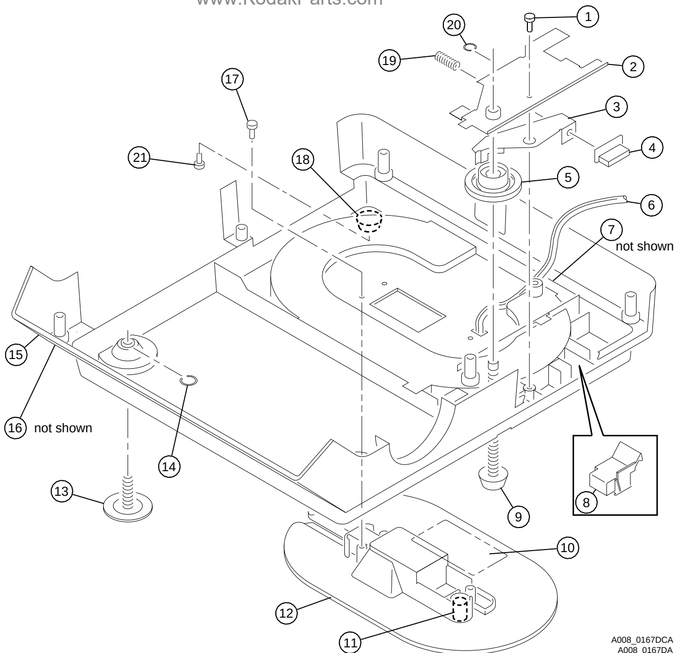
Compliments of: Figure 4 LOWER HOUSING AY www.KodakParts.com
