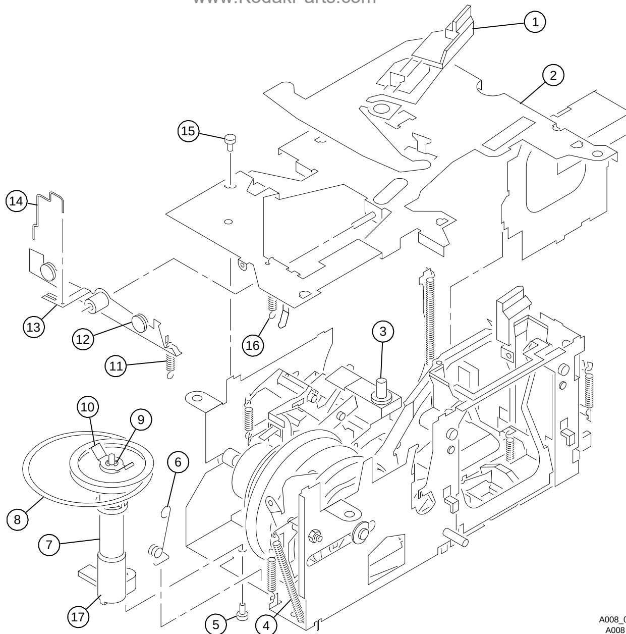
Figure 15 MECHANISM AY/TOP PLATE AY www.KodakParts.com
