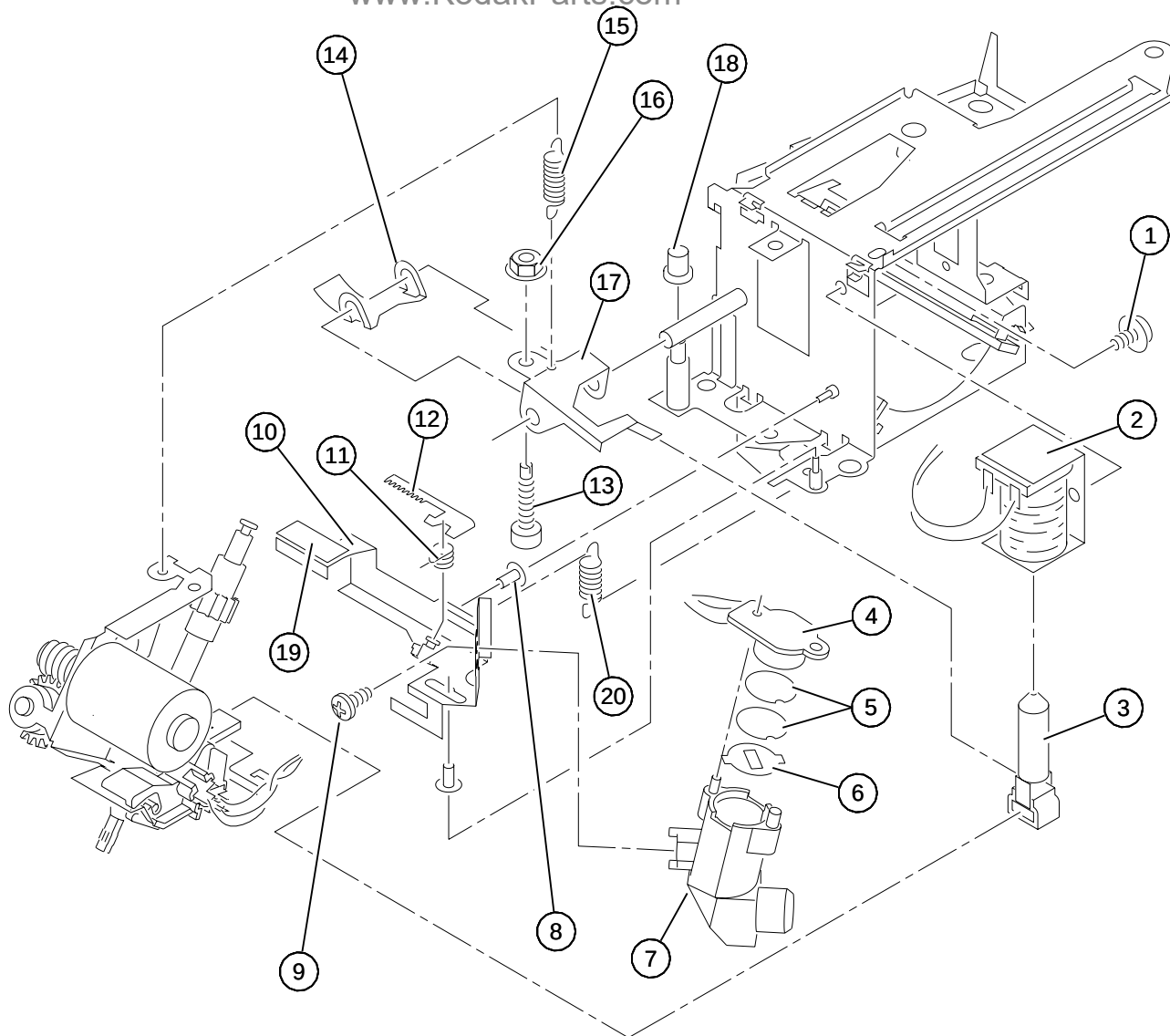
Figure 12 PHOTOCELL/CLAMP PAD AY - III AM/AMT/ATS/III-J AMT/J ATS PROJECTORS Only
