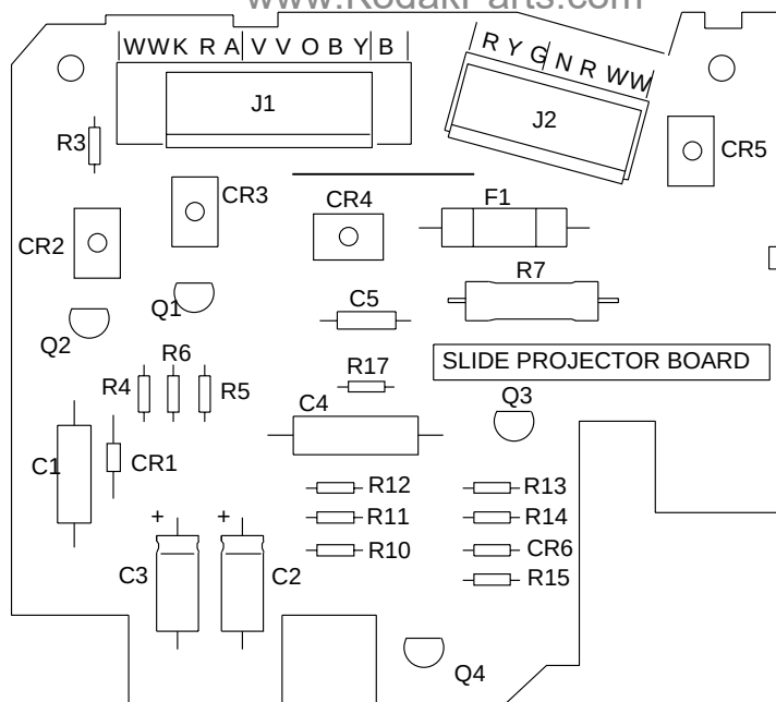
Figure 27 COMPONENT BOARD - III AM/AMT/ATS/III-J AMT/J ATS PROJECTORS Only
