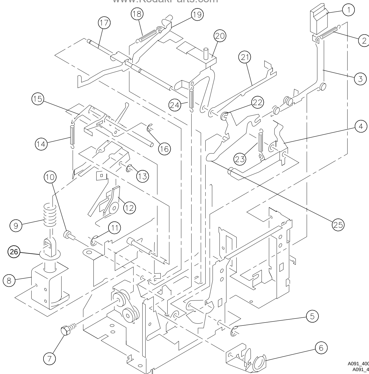
Figure 18 MECHANISM AY/LEVERS www.KodakParts.com
