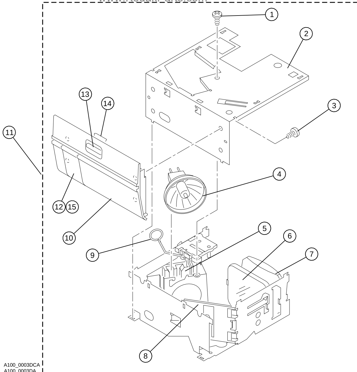
Figure 6 LAMP MODULE AY - Non-Painted www.KodakParts.com
