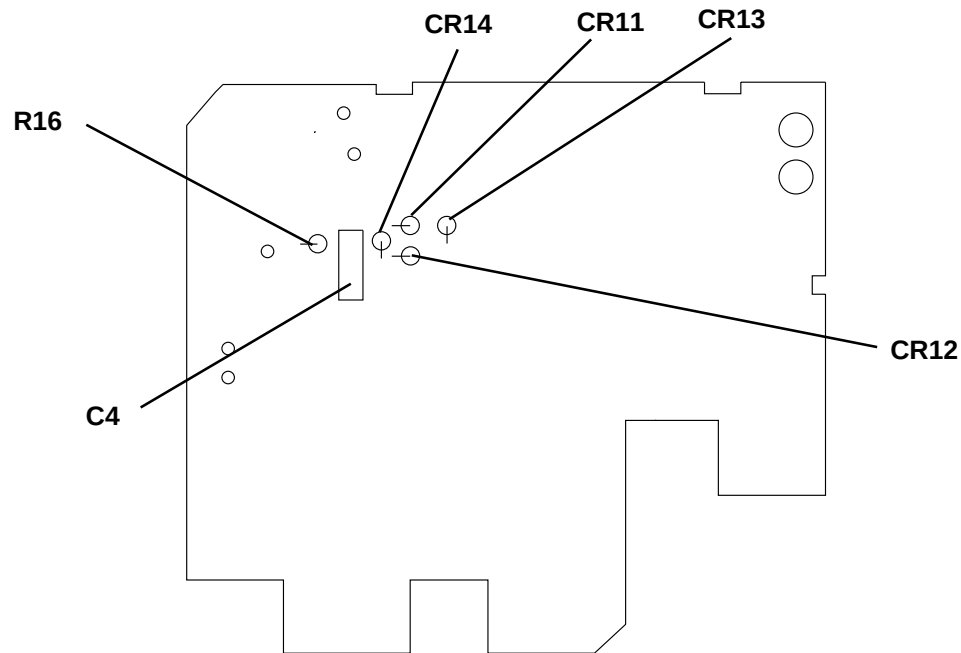
Figure 24 Style 1 COMPONENT BOARD - III E/B/BR PROJECTORS Only
