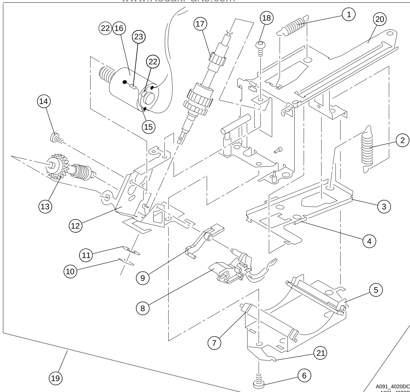
Figure 11 LENS MOUNT AY - AUTO FOCUS PROJECTORS
