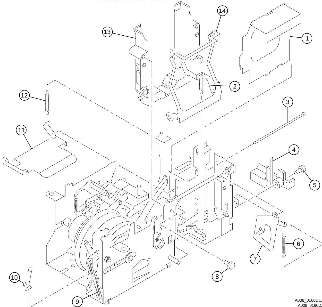
Figure 16 MECHANISM AY/SHUTTER and GATE AY www.KodakParts.com
