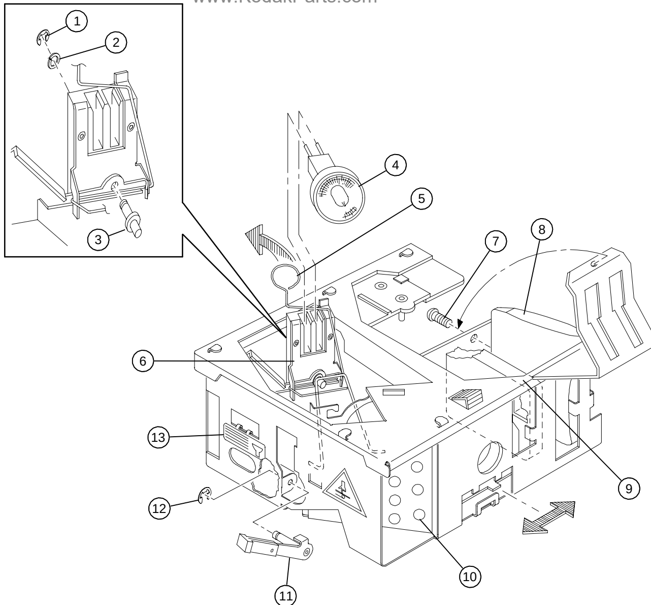
Compliments of: Figure 7 LAMP MODULE AY - Painted www.KodakParts.com
