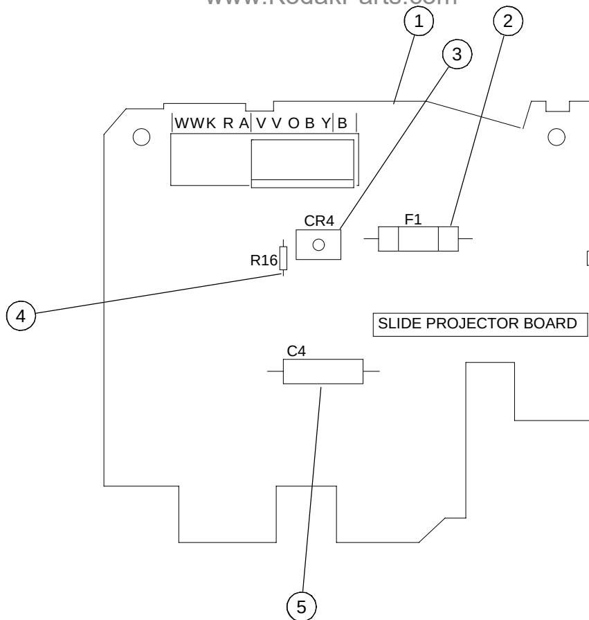
Figure 25 Style 2 COMPONENT BOARD - III B/BR/E/E PLUS/III-J E PLUS/KK E PLUS PROJECTORS Only
