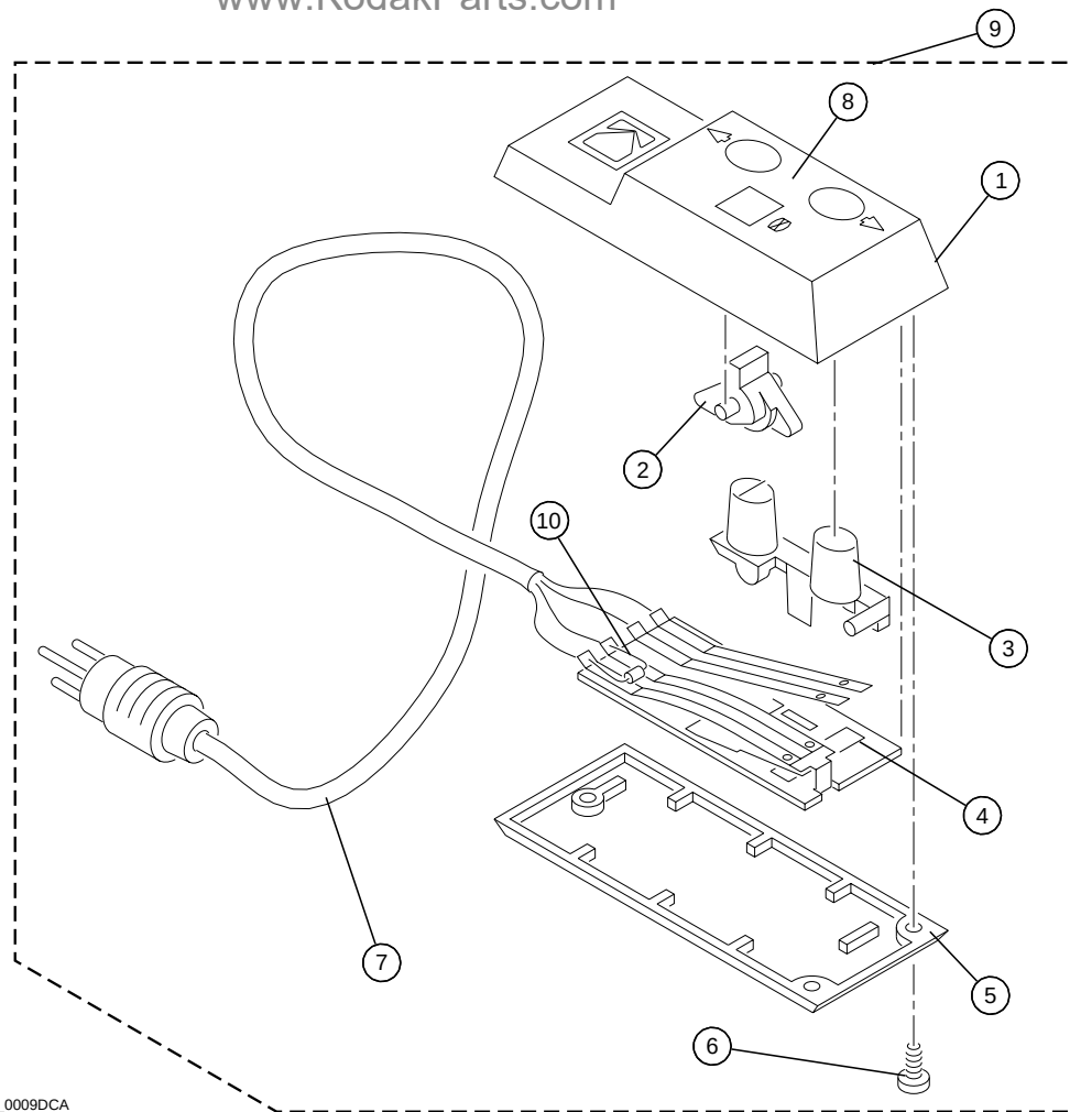
Compliments of: Figure 19 EC2 and EC3 REMOTE CONTROLS www.KodakParts.com
