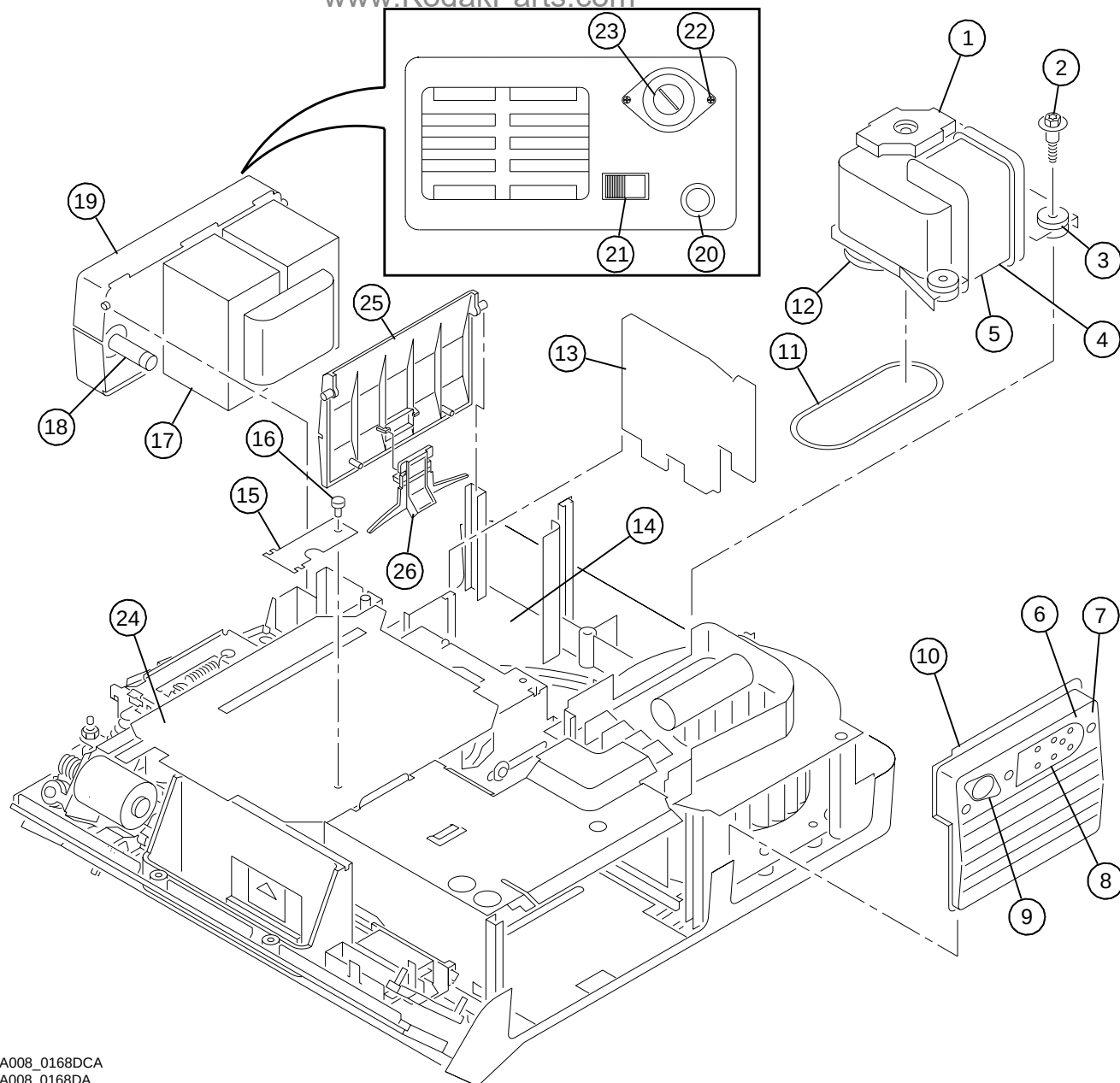
Compliments of: Figure 8 MOTOR and Electrical www.KodakParts.com
