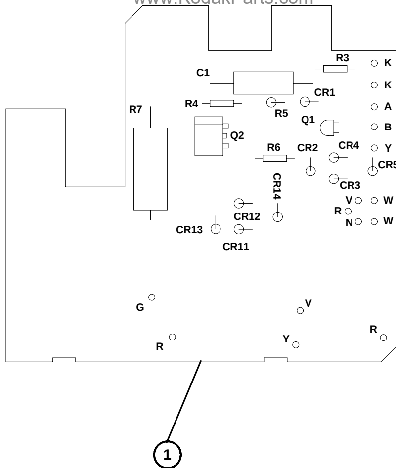
Figure 21 Style 1 COMPONENT BOARD - III A PROJECTORS Only
