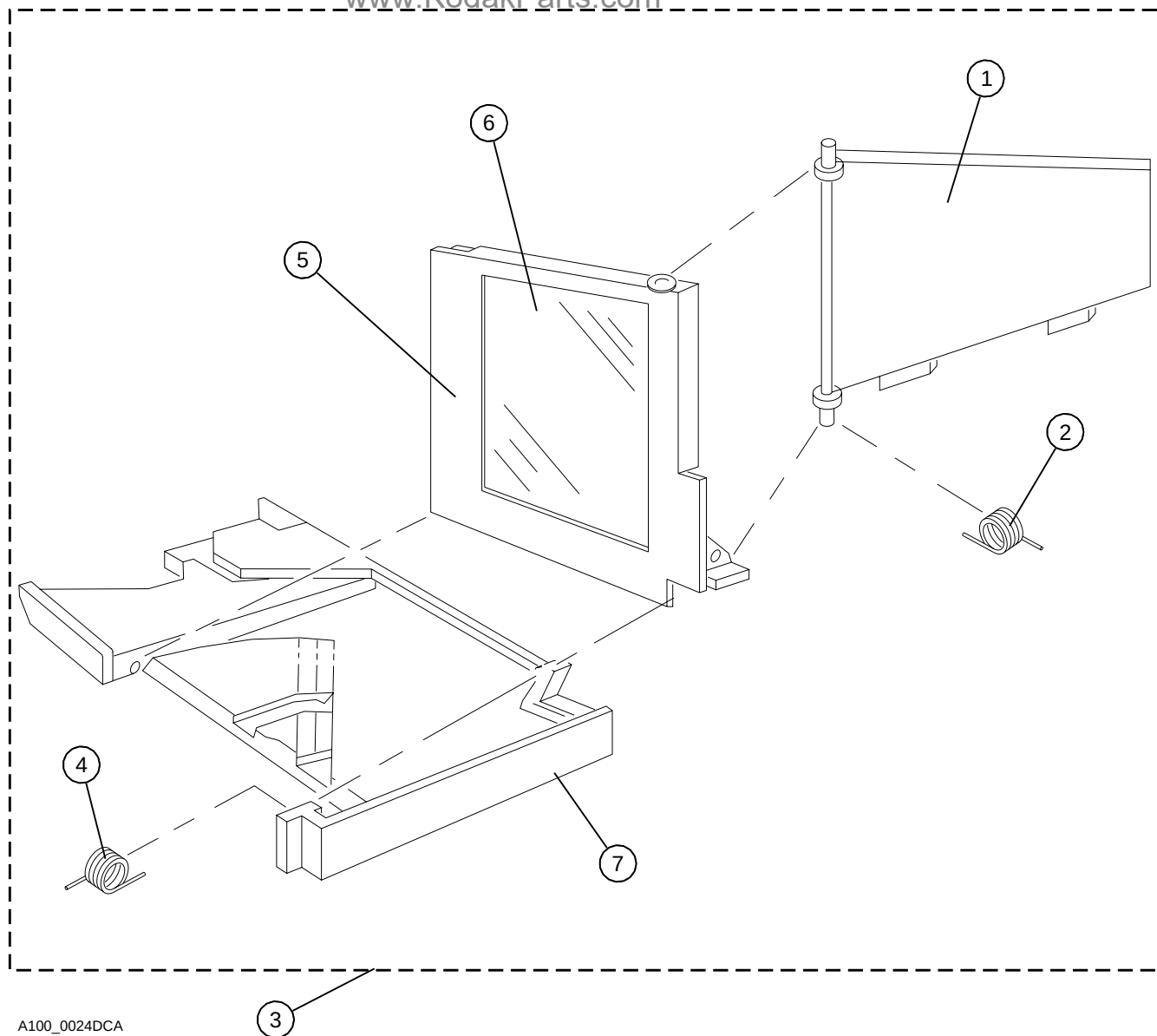
Figure 5 MOUNT MIRROR/VIEWER DRAWER www.KodakParts.com
