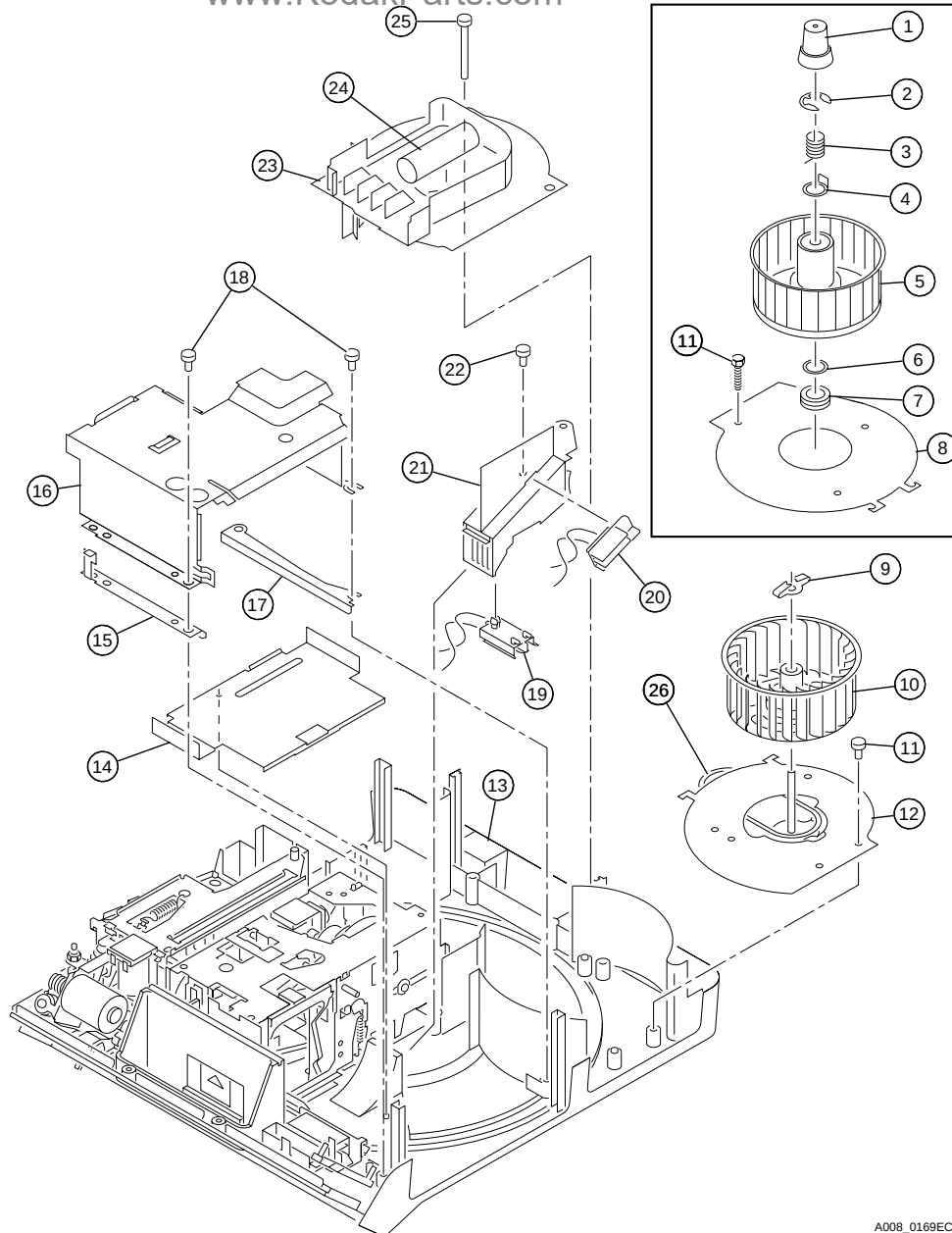
Figure 9 LAMP and COOLING SYSTEM www.KodakParts.com
