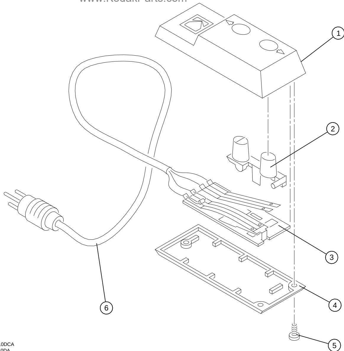
Figure 20 EC1 REMOTE CONTROL for III A/III E/III-J A/III-KK A PROJECTORS Only
