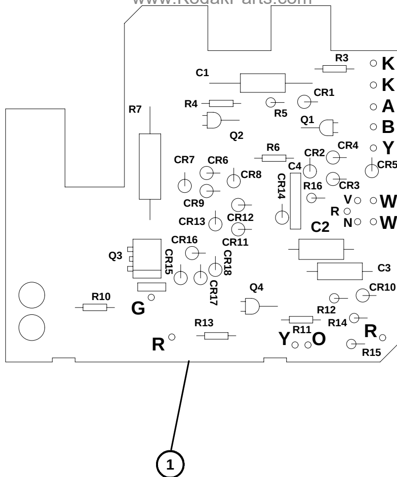
Figure 23 Style 1 COMPONENT BOARD - III ATS PROJECTORS Only
