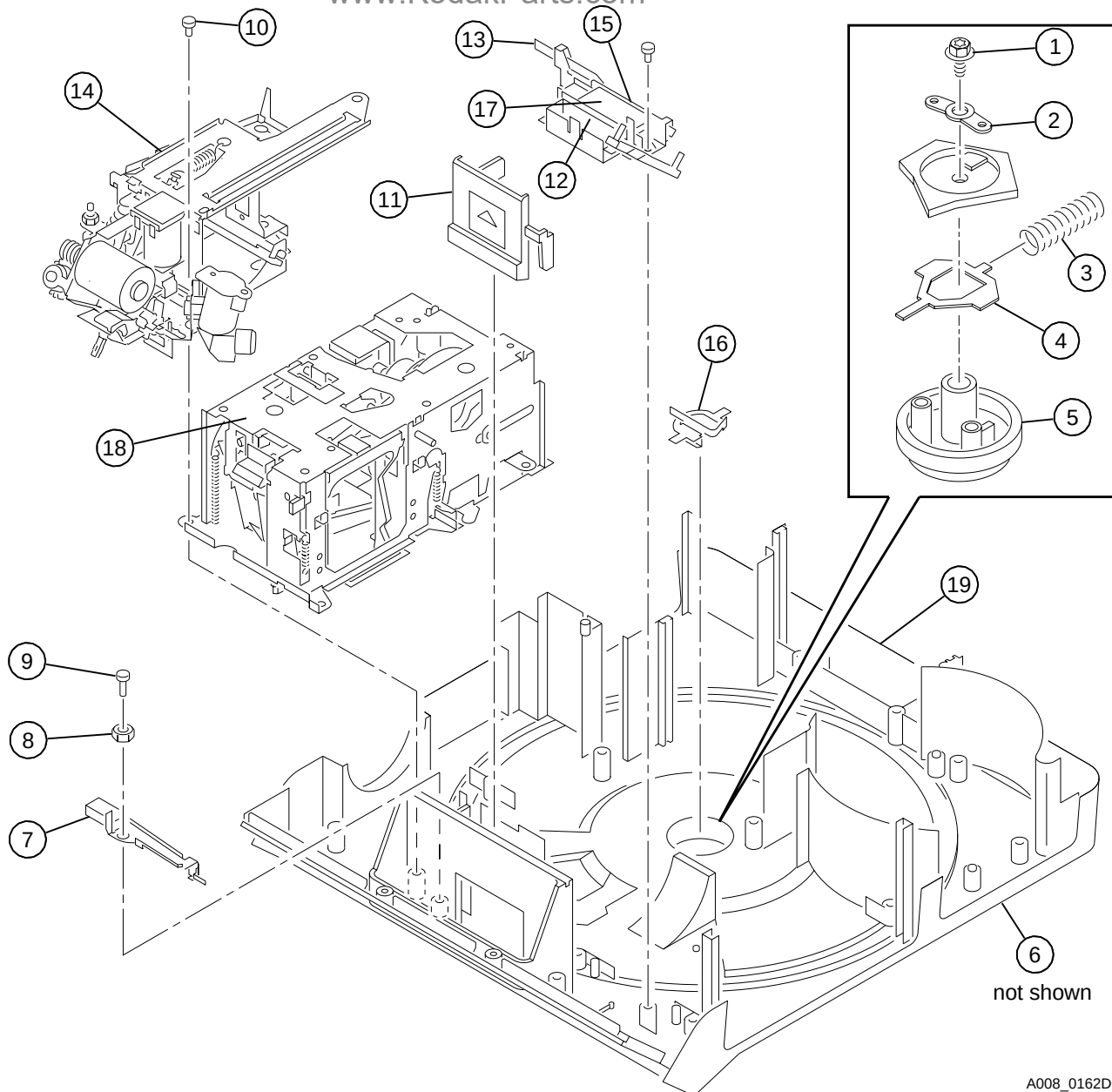
Figure 14 MECHANISM AY and TOP HOUSING AY www.KodakParts.com
