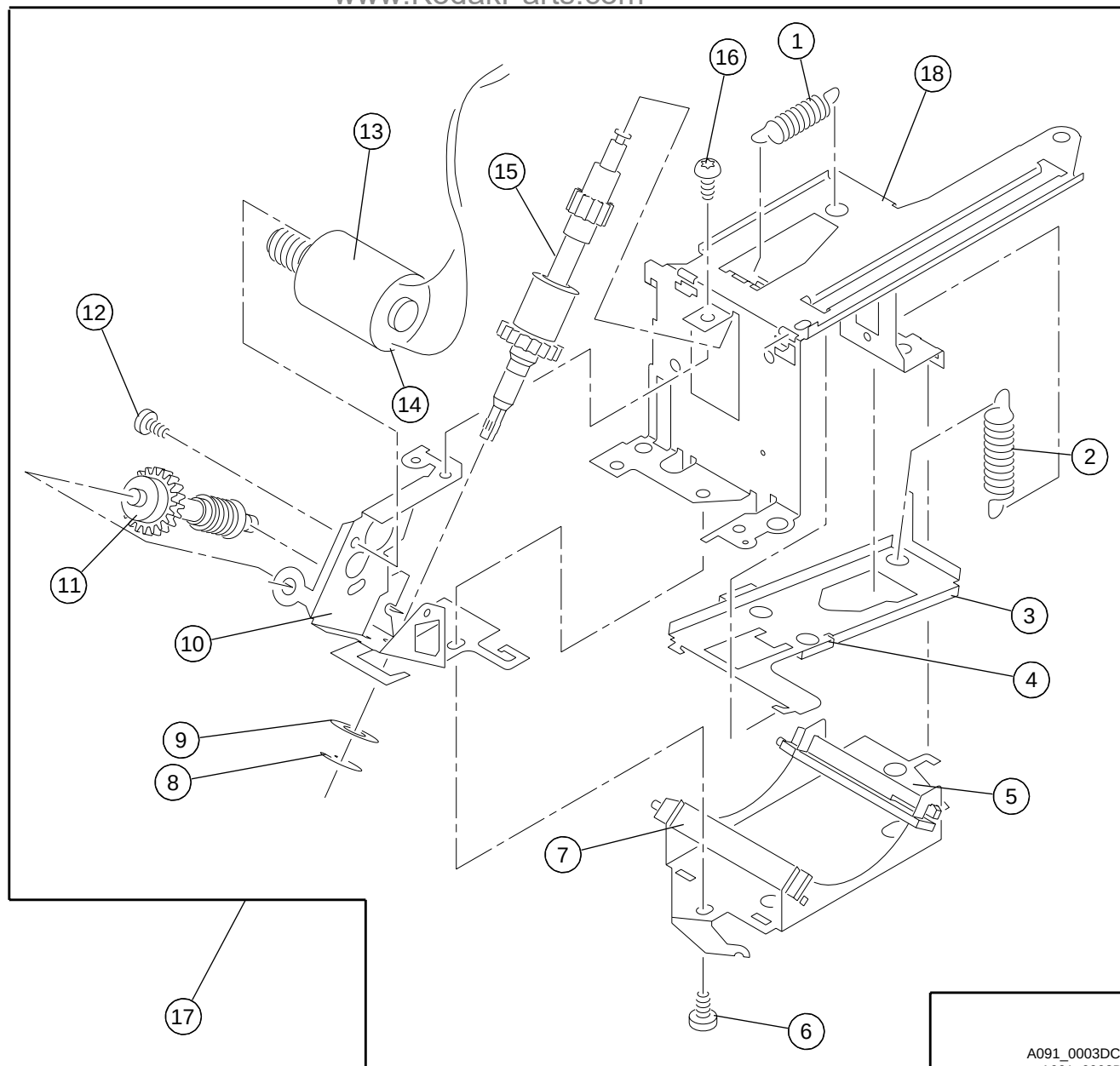
Figure 10 LENS MOUNT AY - NON AUTO FOCUS PROJECTORS
