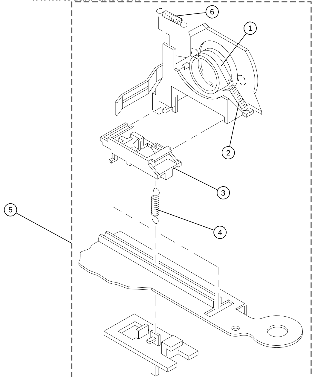
Figure 13 VIEWER FOCUS ADJUSTMENT www.KodakParts.com
