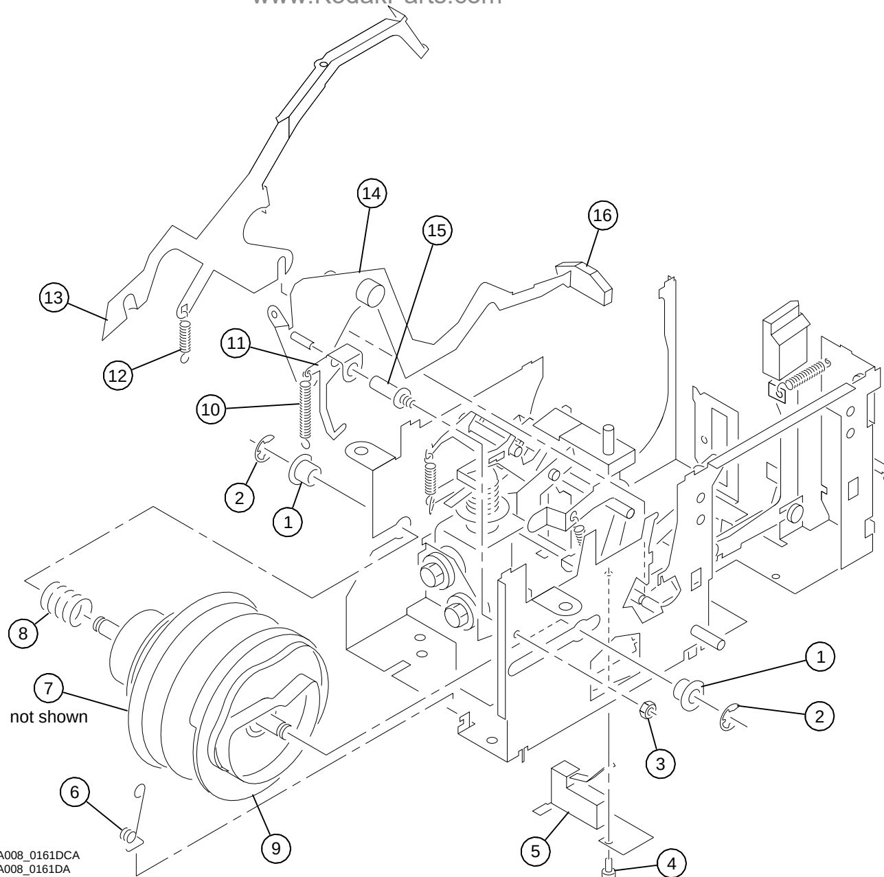
Figure 17 MECHANISM AY/CAMSTACK AY www.KodakParts.com
