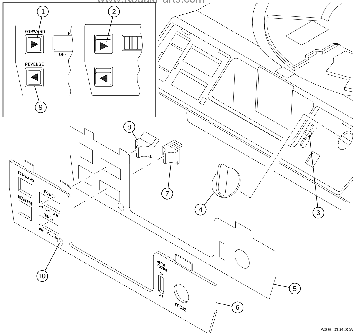
Figure 3 CONTROL PANEL www.KodakParts.com
