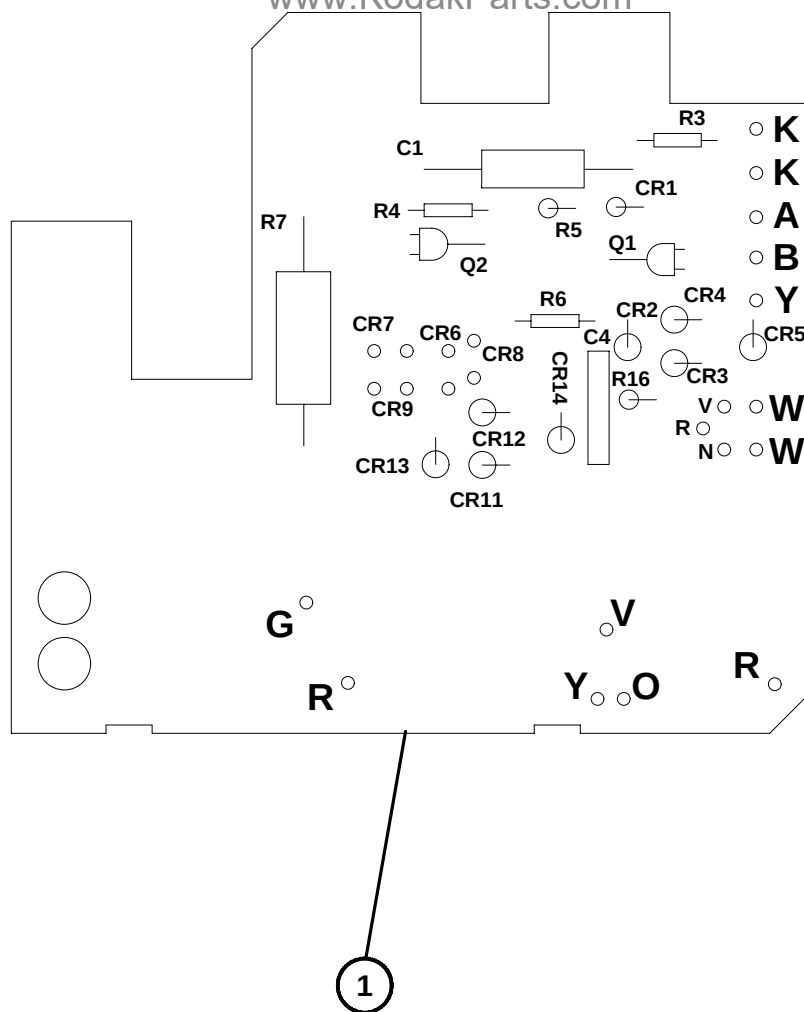
Figure 22 Style 1 COMPONENT BOARD - III AM PROJECTORS Only
