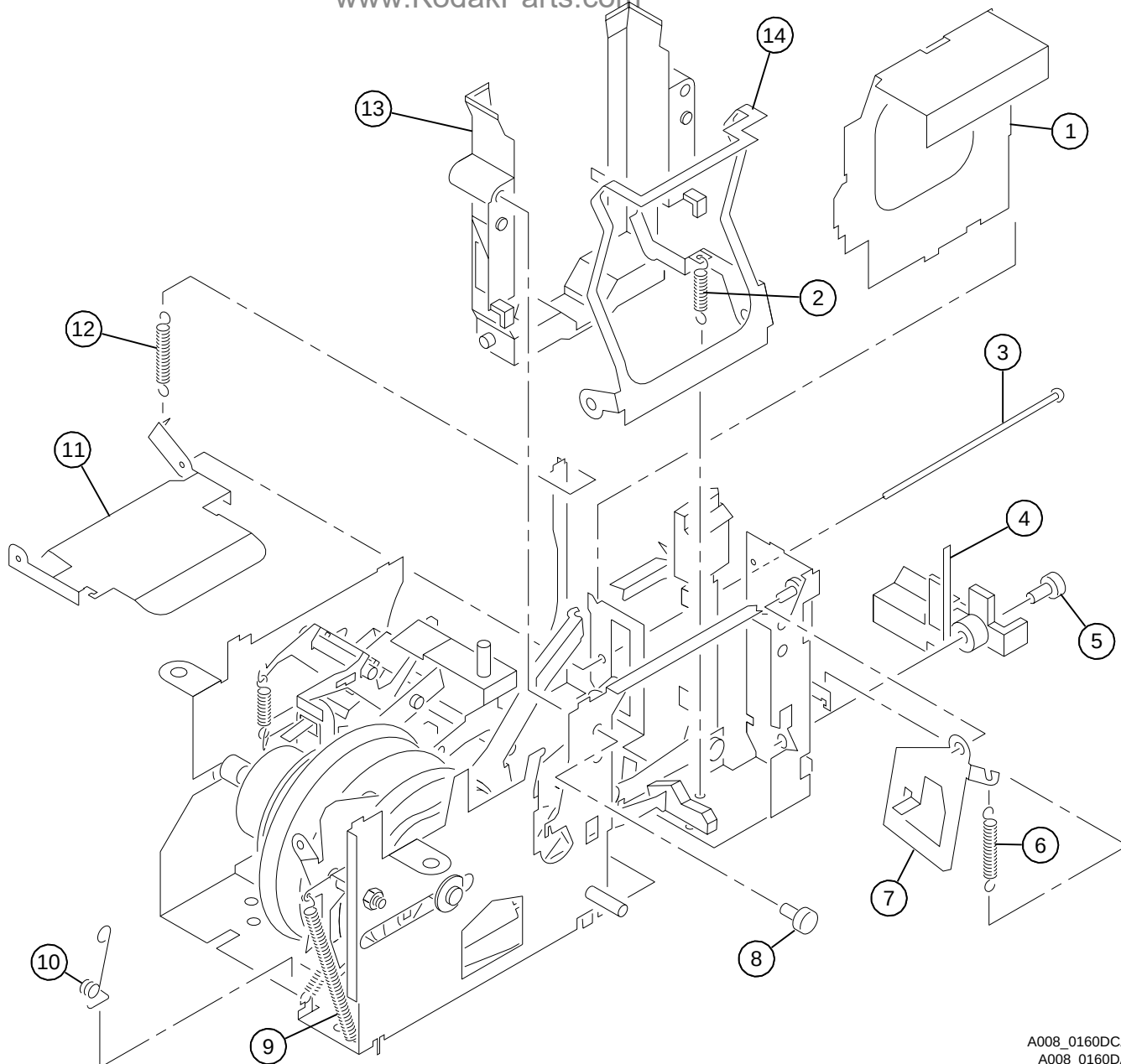
Figure 18 MECHANISM, SHUTTER and GATE ASSEMBLIES
