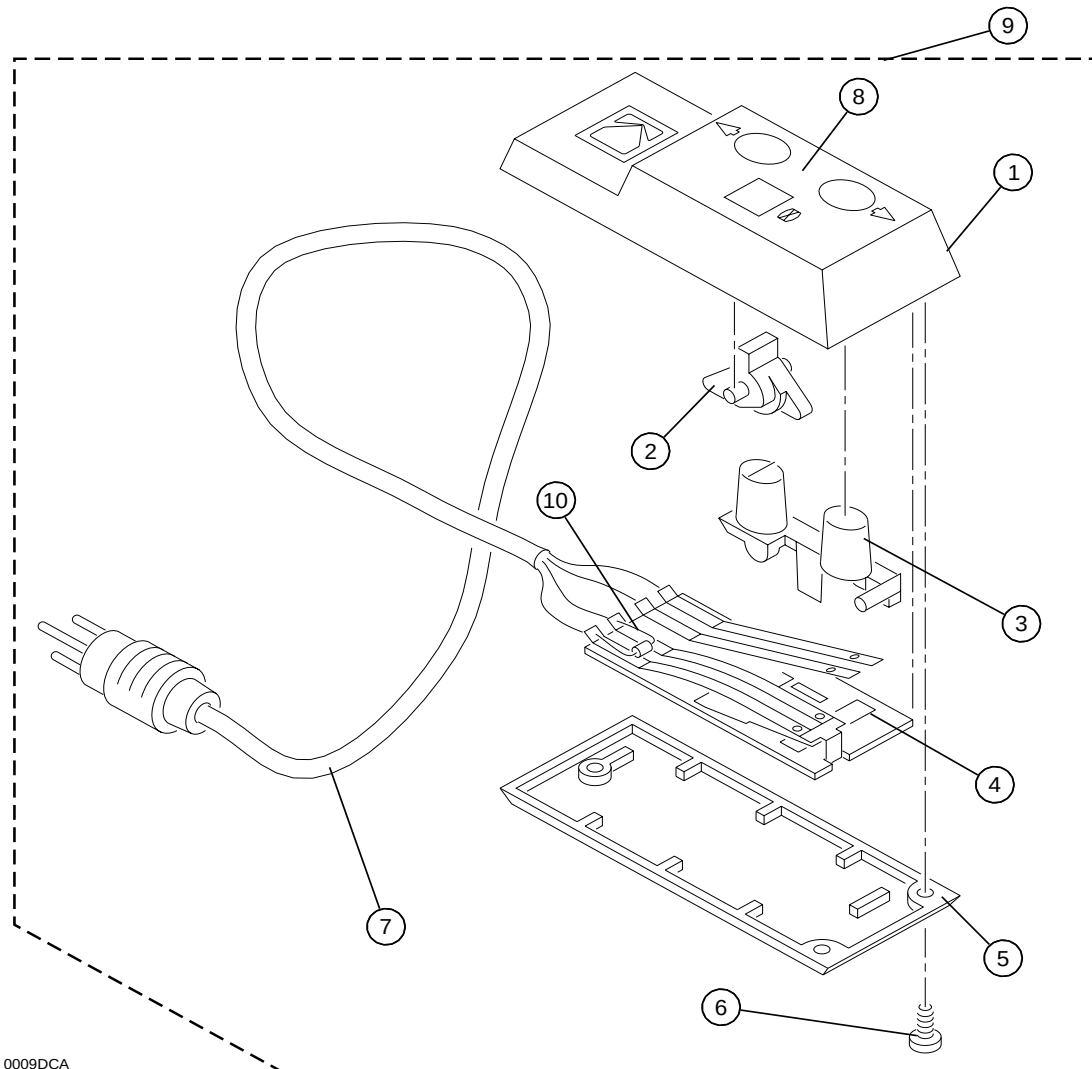
Figure 21 REMOTE CONTROL EC2 for the 4400 PROJECTOR and REMOTE CONTROL EC3 for 5600, 5600-KK, 5600-J, I and II PROJECTORS
