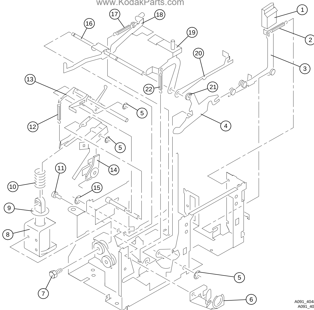
Figure 20 MECHANISM AY and LEVERS www.KodakParts.com
