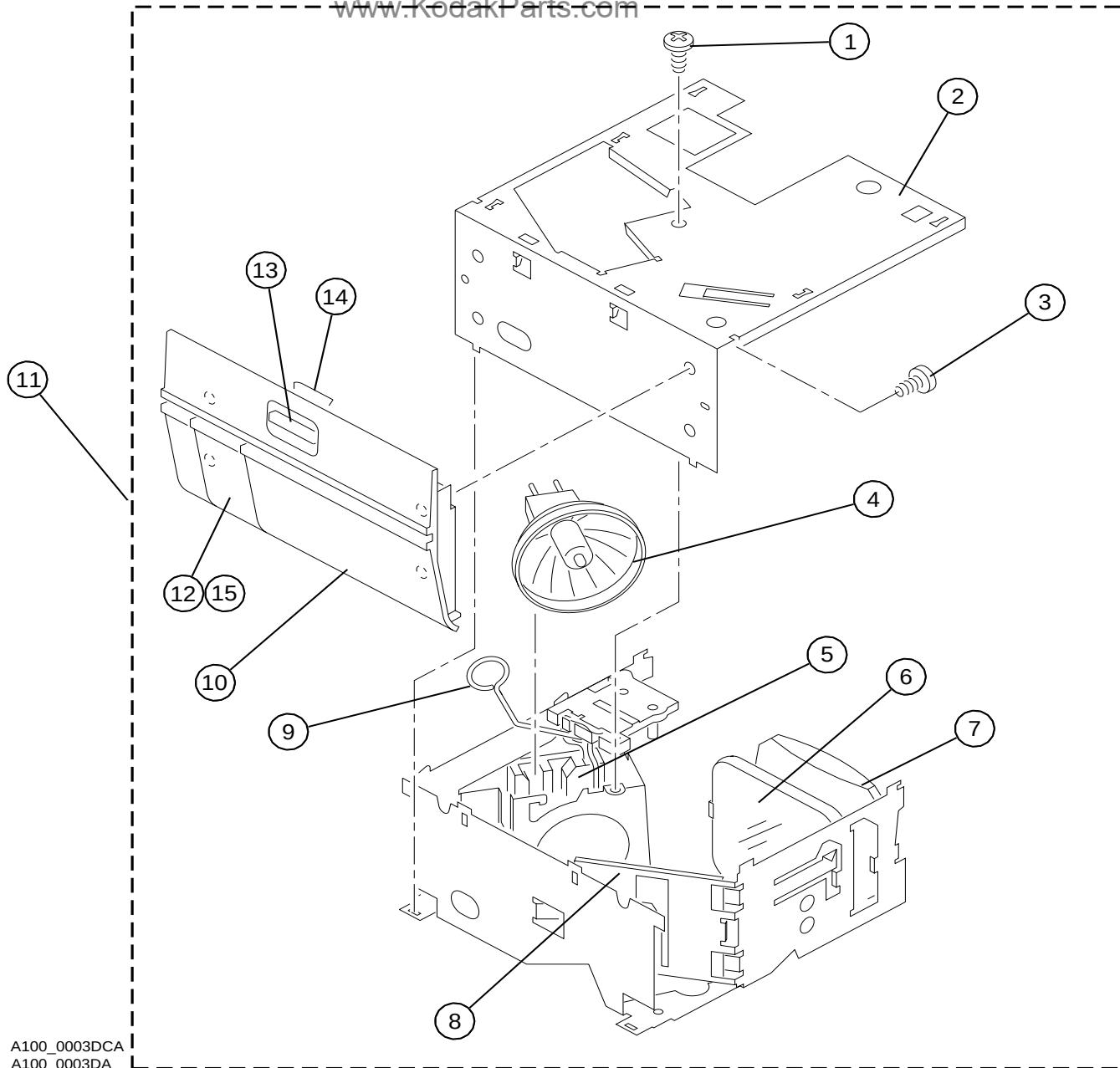
Figure 7 LAMP MODULE AY - Non-Painted
