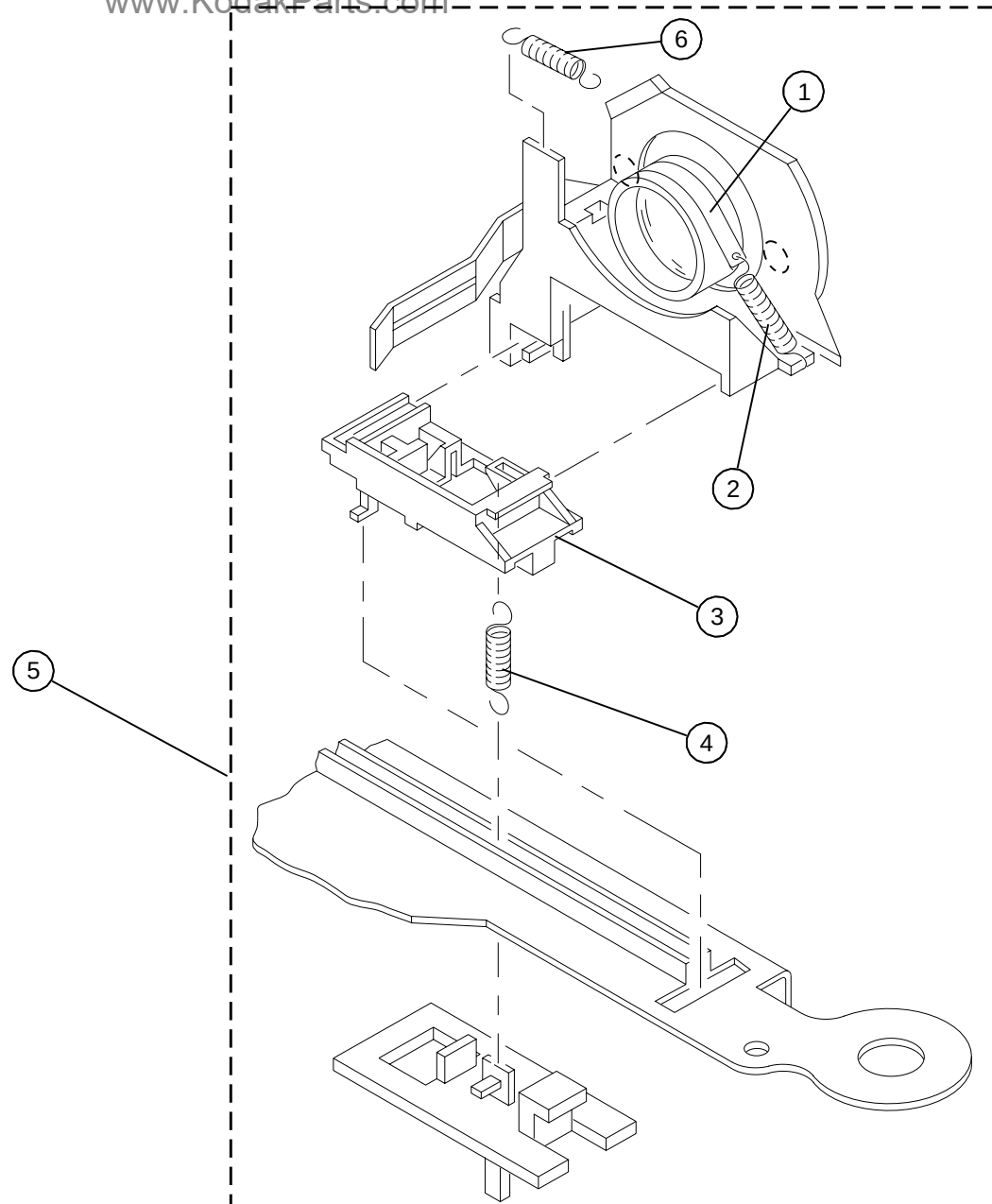
Figure 14 VIEWER FOCUS ADJUSTER www.KodakParts.com
