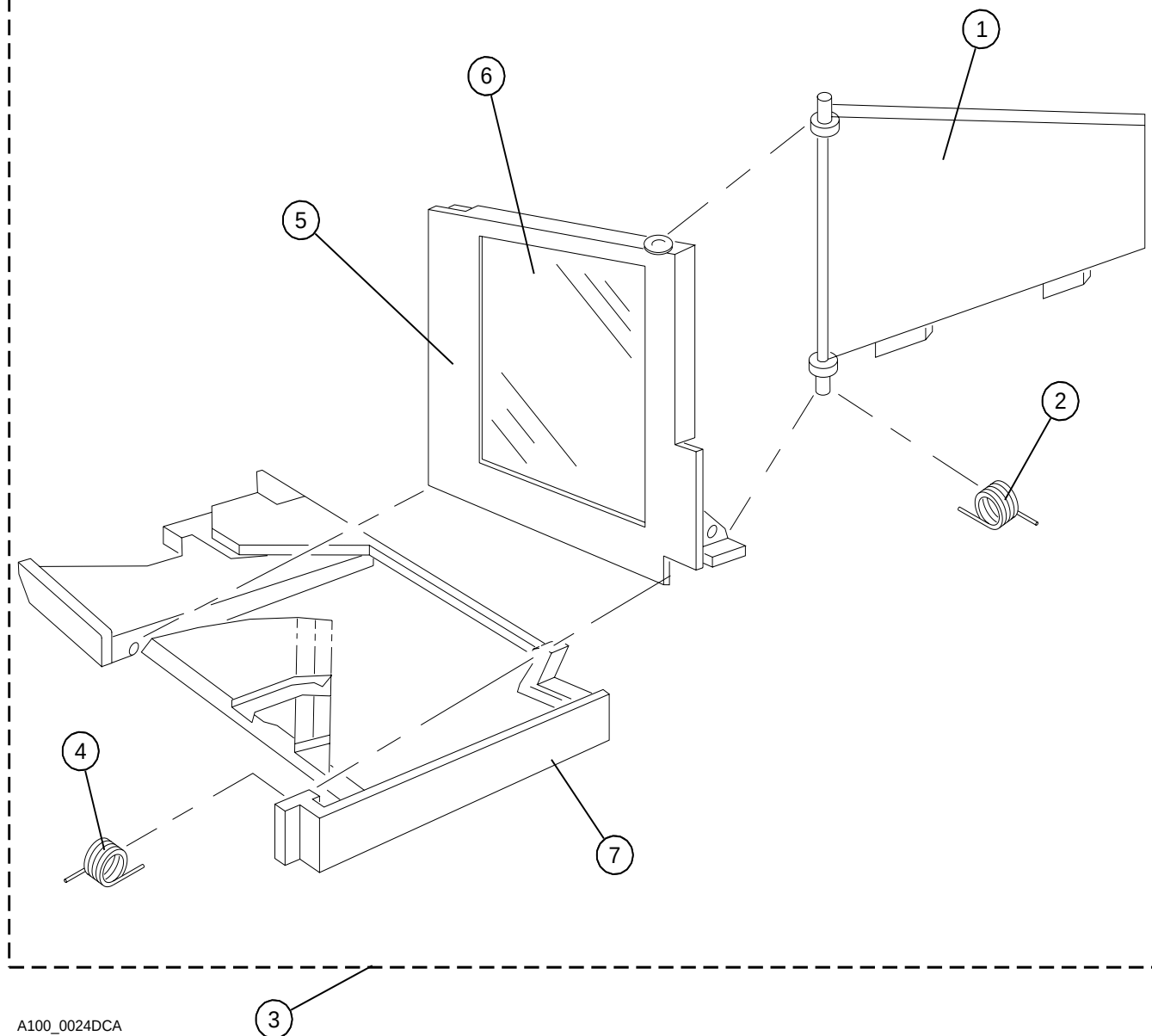
Figure 5 MOUNT MIRROR and VIEWER DRAWER www.KodakParts.com
