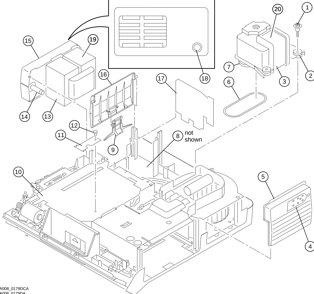
Compliments of: Figure 9 MOTOR and ELECTRICAL www.KodakParts.com
