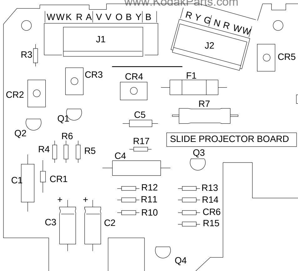
Figure 28 COMPONENT BD - Style 2 for 5400, 5600, 5600-J, 5600-KK, and II PROJECTORS
