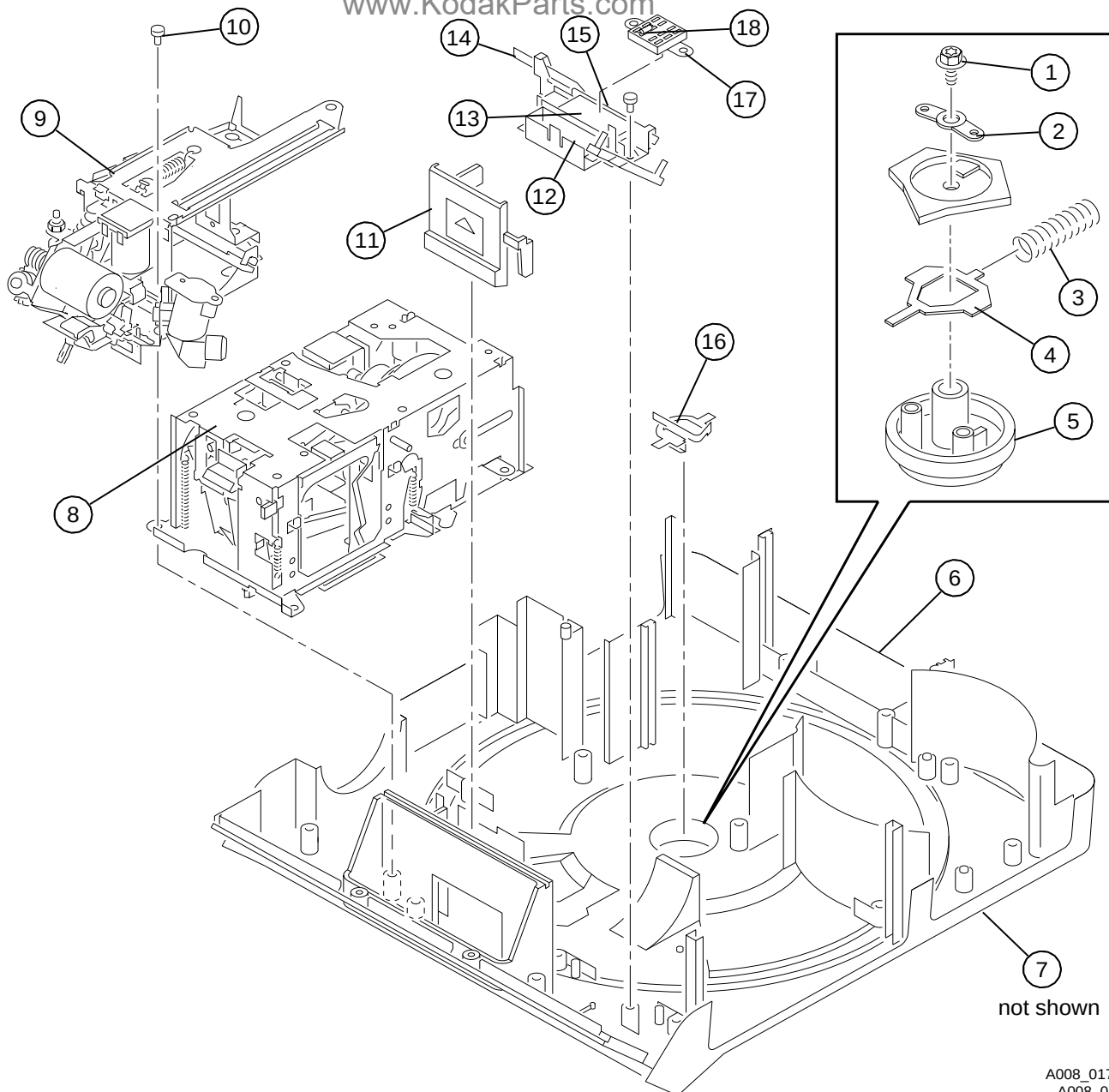
Figure 15 MECHANISM and TOP HOUSING ASSEMBLIES
