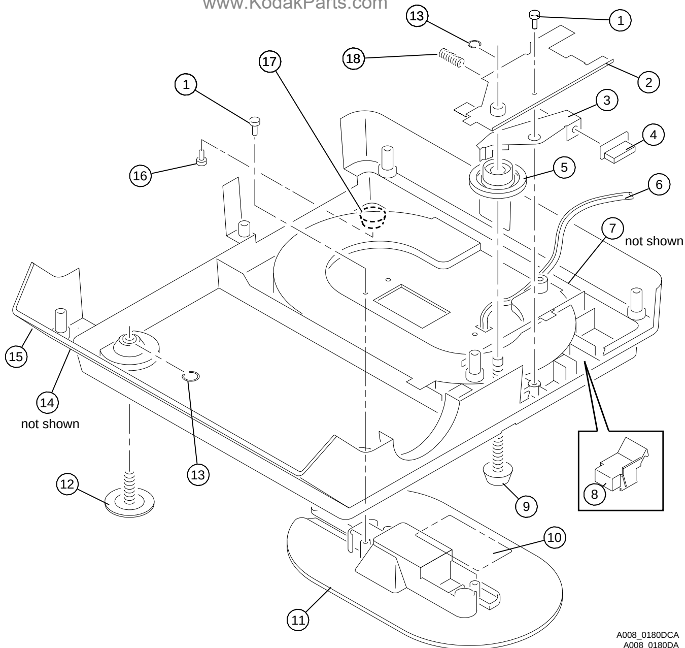
Figure 4 LOWER HOUSING AY www.KodakParts.com
