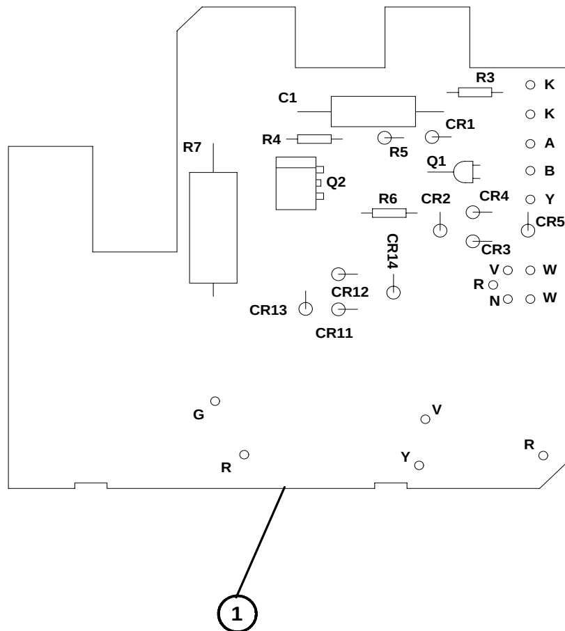
Figure 23 COMPONENT BD - Style 1 for PROJECTORS 4600, 4600-K, 4600-KK, 5200, 5200-K, 5400, AF, and PROJECTORS
