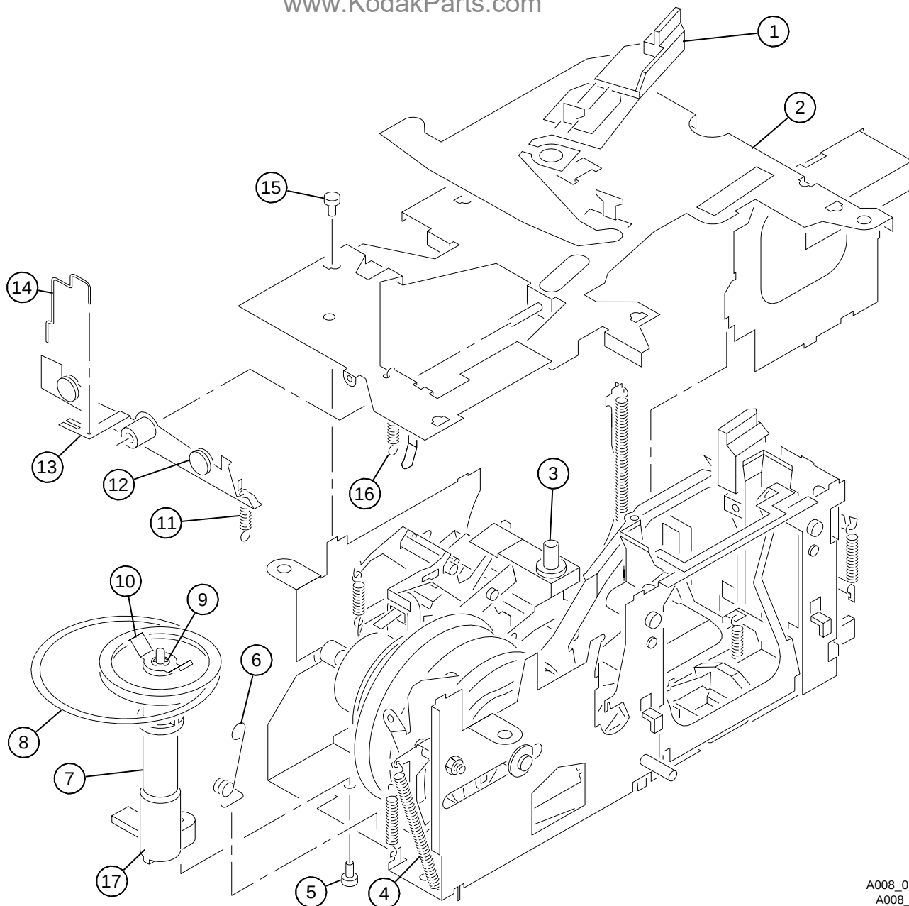
Figure 17 MECHANISM and TOP PLATE ASSEMBLIES www.KodakParts.com
