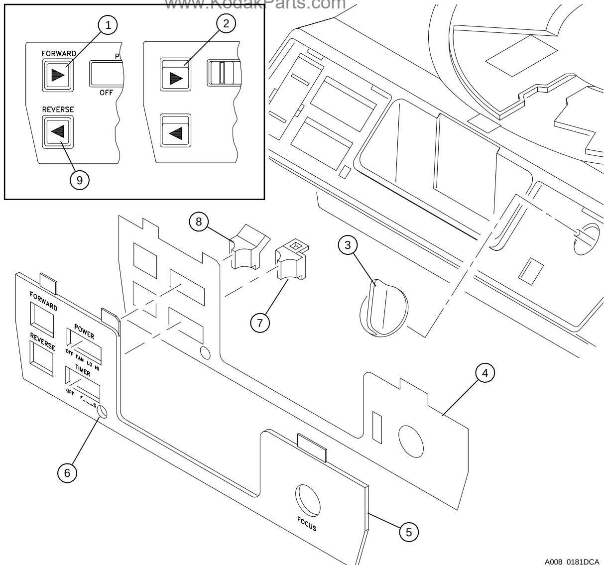
Figure 3 CONTROL PANEL www.KodakParts.com
