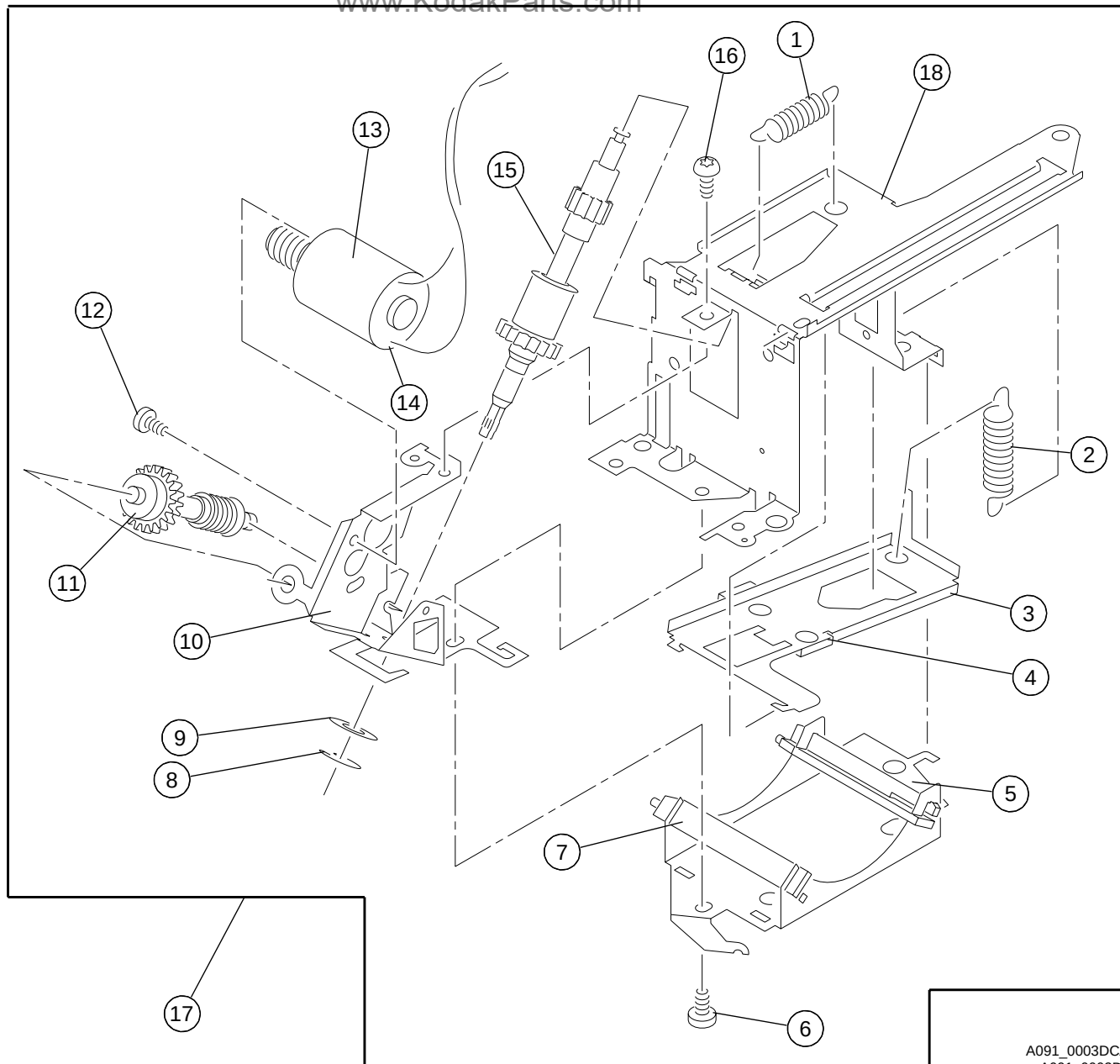
Figure 11 LENS MOUNT AY without AUTO FOCUS
