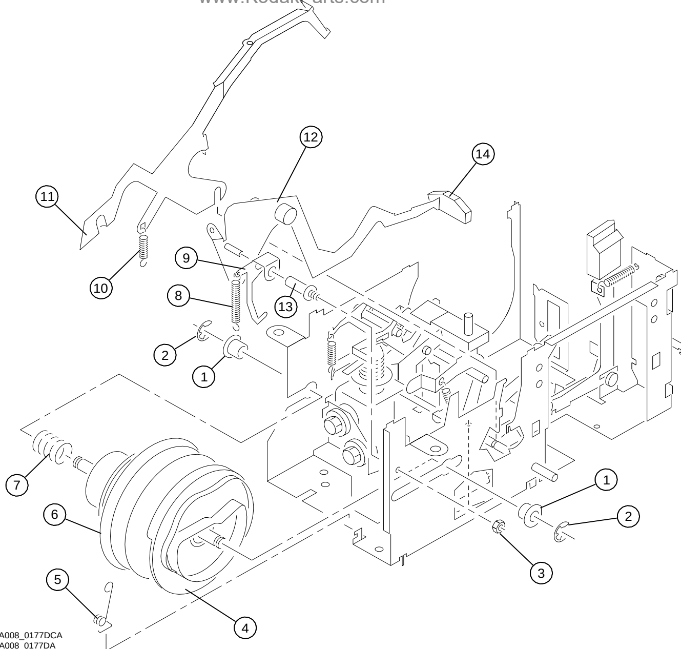
Figure 19 MECHANISM and CAMSTACK ASSEMBLIES www.KodakParts.com
