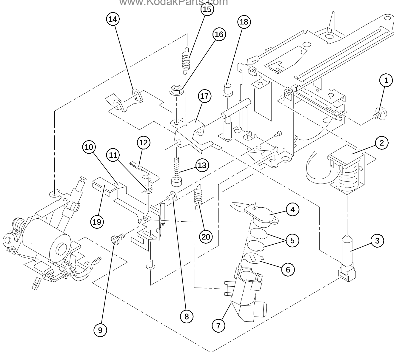
Figure 13 PHOTOCELL and CLAMP PAD AY - 5600, 5600-J, 5600-KK, and II PROJECTORS
