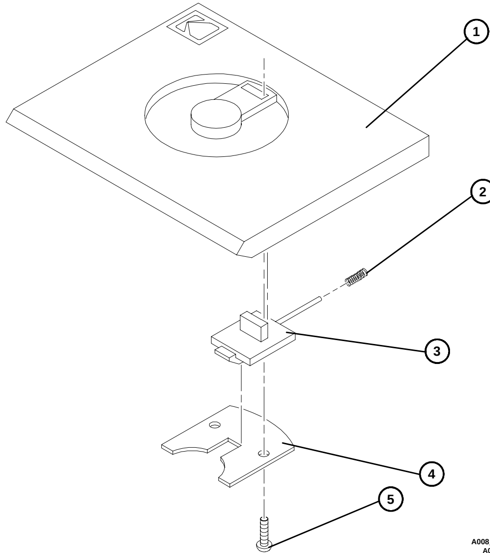
Figure 16 DUST COVER www.KodakParts.com
