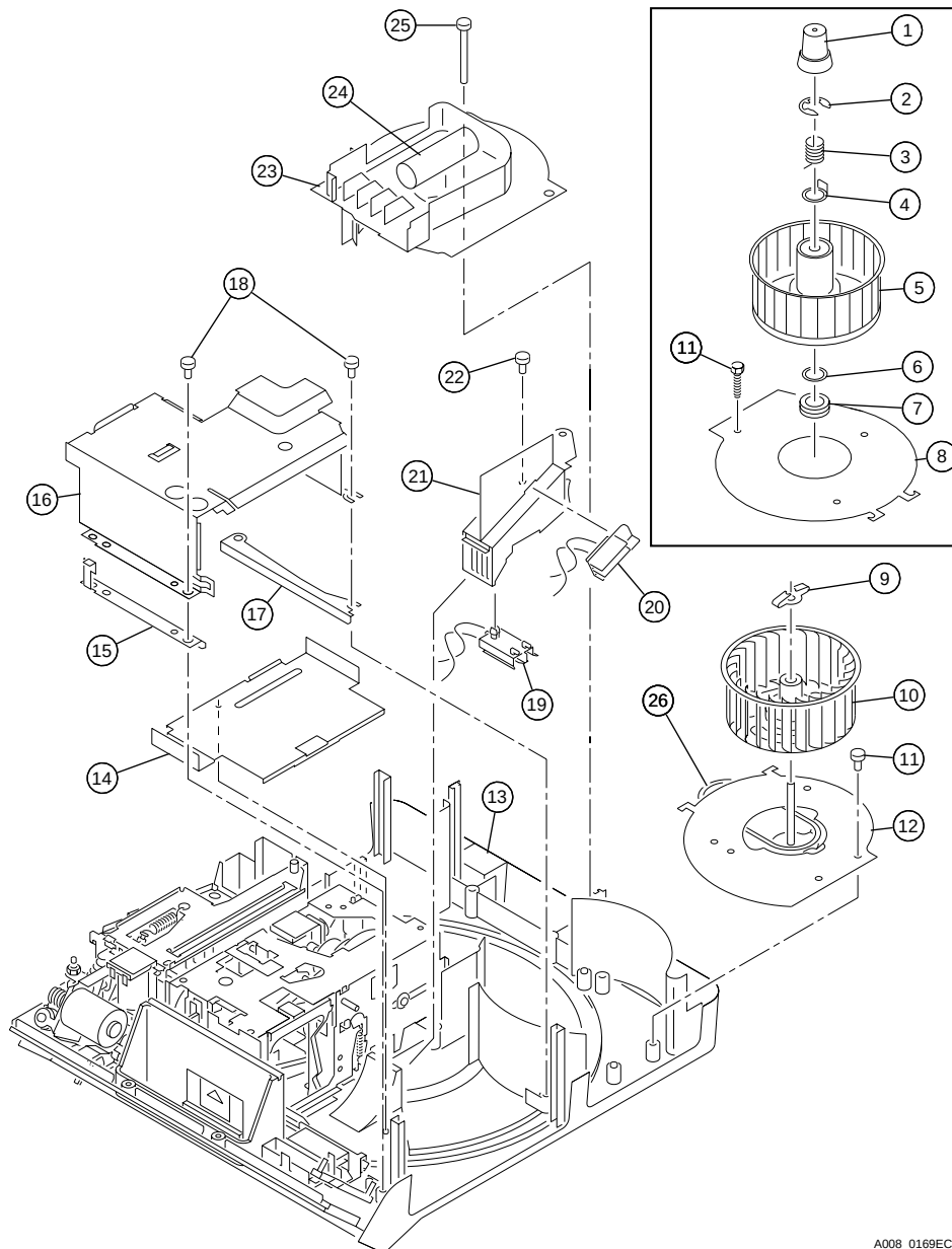
Figure 10 LAMP and COOLING SYSTEM www.KodakParts.com
