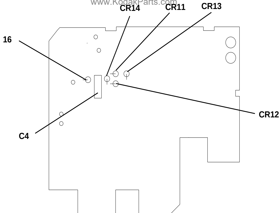
Figure 25 COMPONENT BD - Style 1 for 4200, 4200-J, 4200-K, 4200-KK, and 4400 PROJECTORS
