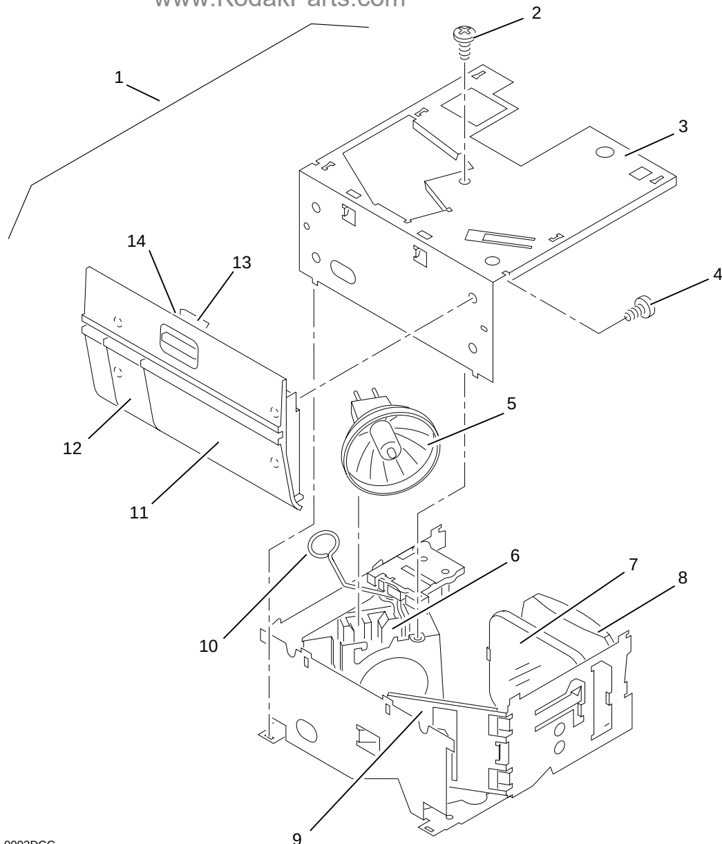
Figure 6 LAMP MODULE AY - High Brightness www.KodakParts.com
