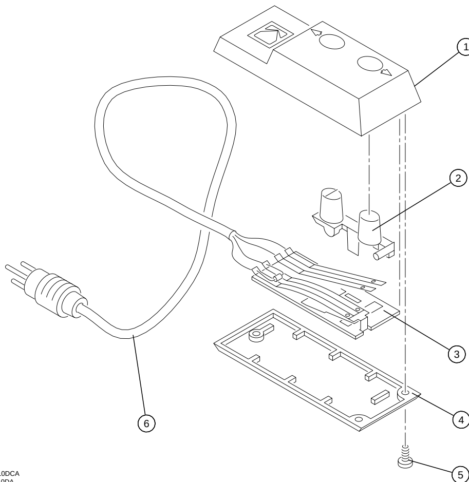
Figure 22 REMOTE CONTROL EC1 for 4200, 4200-K, 4200-KK, 4200-J, 4600, 4600-K, 4600-KK, 5200, 5200-K, 5400, AF, and I PROJECTORS
