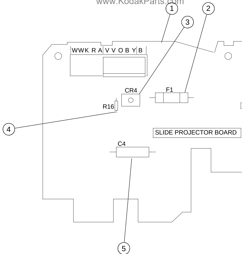
Figure 26 COMPONENT BD - Style 2 for 4200, 4200-J, 4200-K, 4200-KK, and 4400 PROJECTORS
